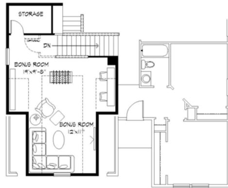
(Opt. Bonus Room) Upper Level Floor
